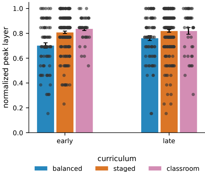
Peak-encoding depth by curriculum
